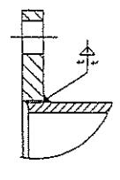
NOZZLE TO FLANGE WELD JOINTS
